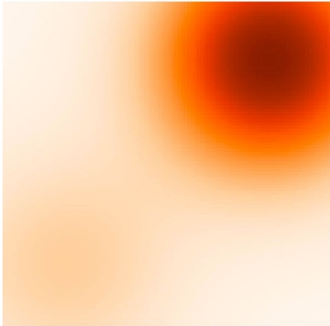
Perturbed density
