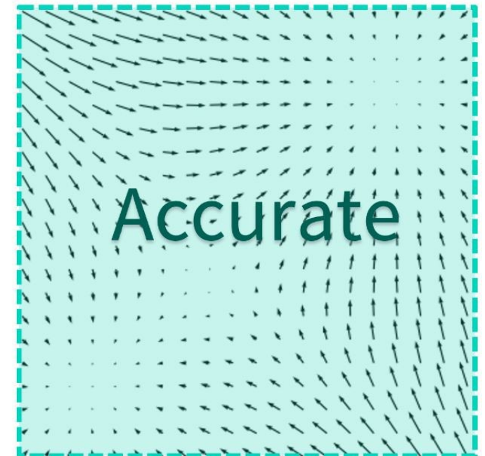
Estimated scores
