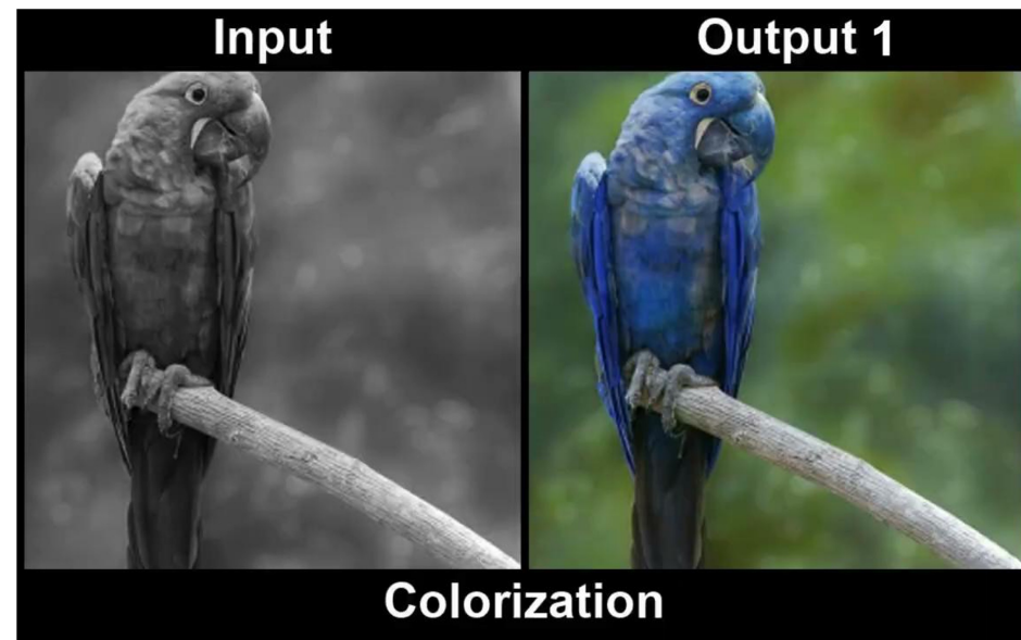
Colorization
