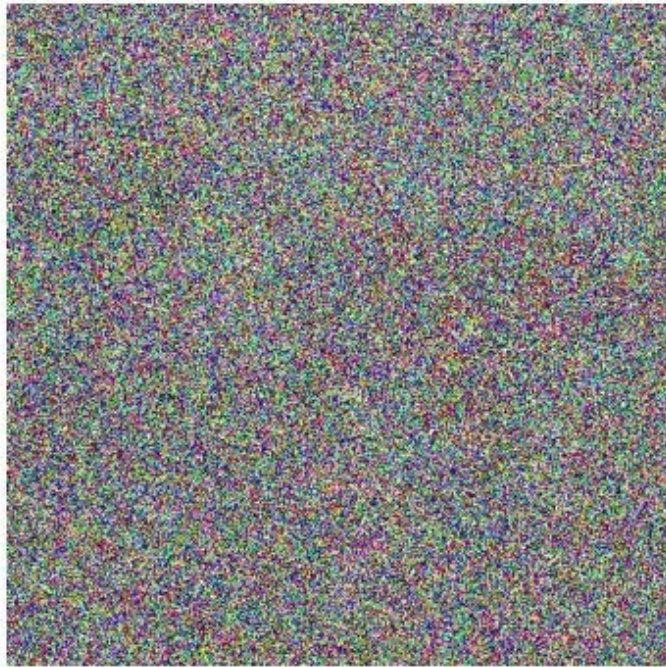
Many Steps
