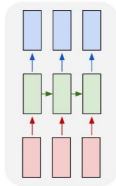
e.g. Video classification on frame level
