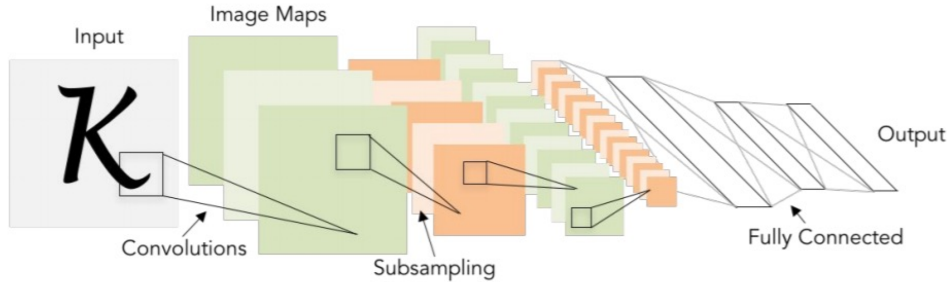
LeNet-5
