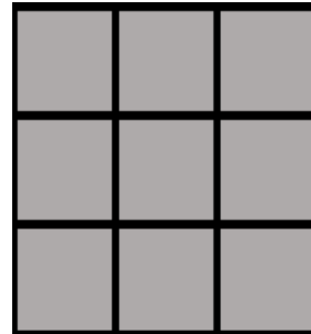
3x3 filter
