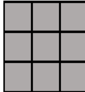
3x3 filter
