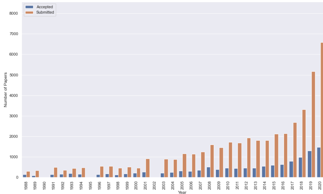
CVPR papers
