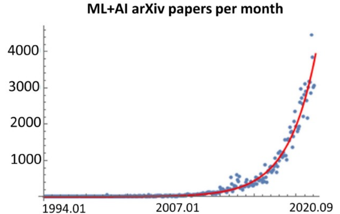
ML+AI papers
